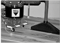
[CASTOR CHAIR TEST] ISO 4918 198 lbs. castor chair test performed to check for flooring breaks and transfers.
